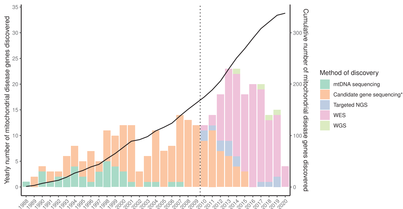
Fig. 2. Methods of disease gene discovery. Demonstration of the shift from mt-DNA and candidate gene sequencing to NGS, marked by the dashed lined in 2010, and reflected by an acceleration in disease gene discovery. Studies marked with an asterisk include a combination of linkage analysis, homozygosity mapping, and candidate gene sequencing.
